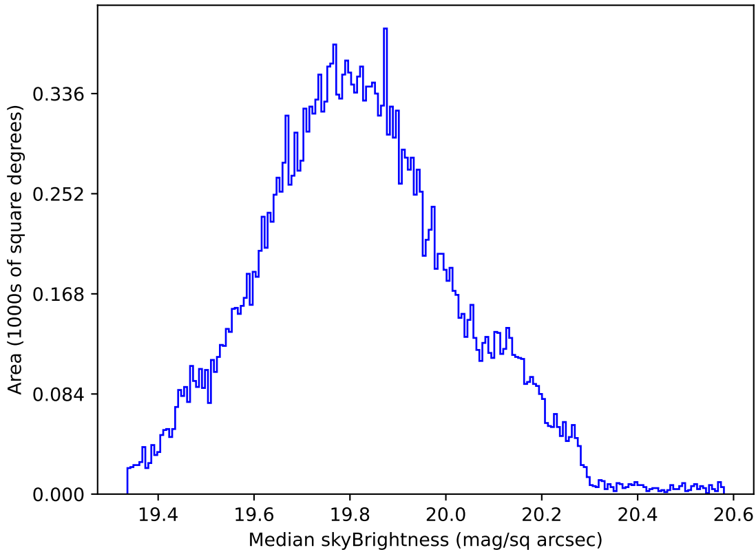
roll_pause_mjdp0_v3.4_10yrs All sky all bands: Median skyBrightness
