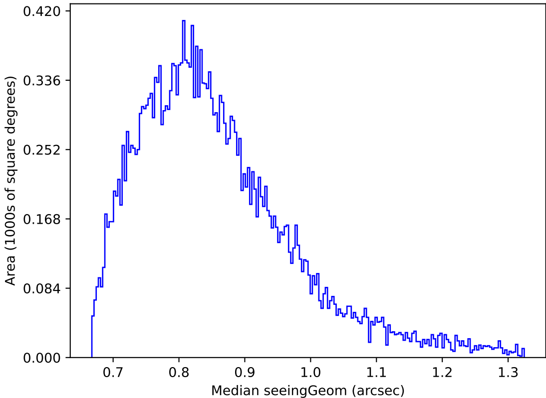
roll_pause_mjdp0_v3.4_10yrs Yr 1 z band: Median seeingGeom
