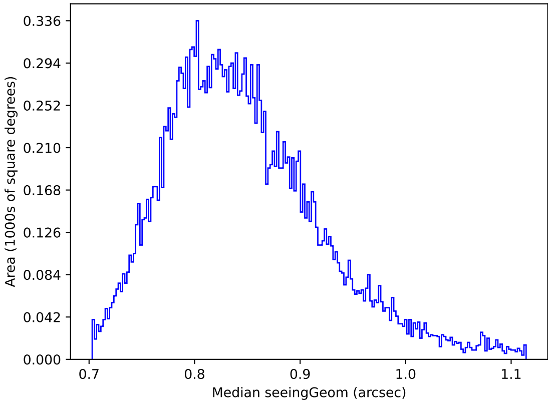
roll_pause_mjdp0_v3.4_10yrs Yr 1 y band: Median seeingGeom
