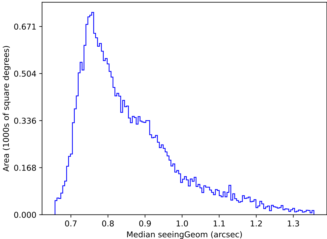
roll_pause_mjdp0_v3.4_10yrs Yr 1 r band: Median seeingGeom
