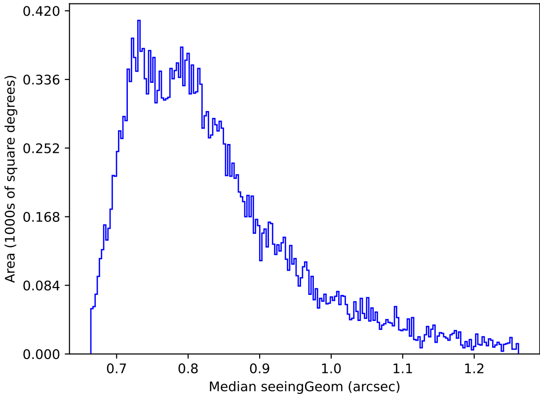
roll_pause_mjdp0_v3.4_10yrs Yr 1 i band: Median seeingGeom
