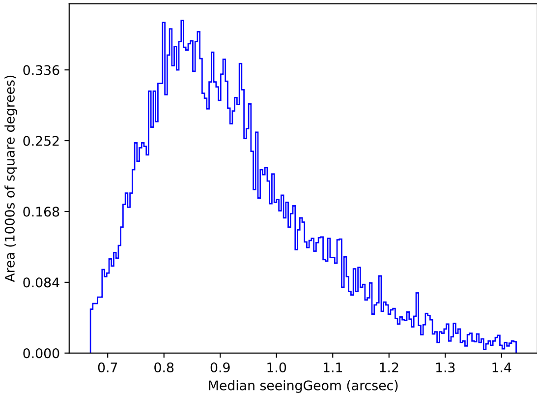
roll_pause_mjdp0_v3.4_10yrs Yr 1 g band: Median seeingGeom
