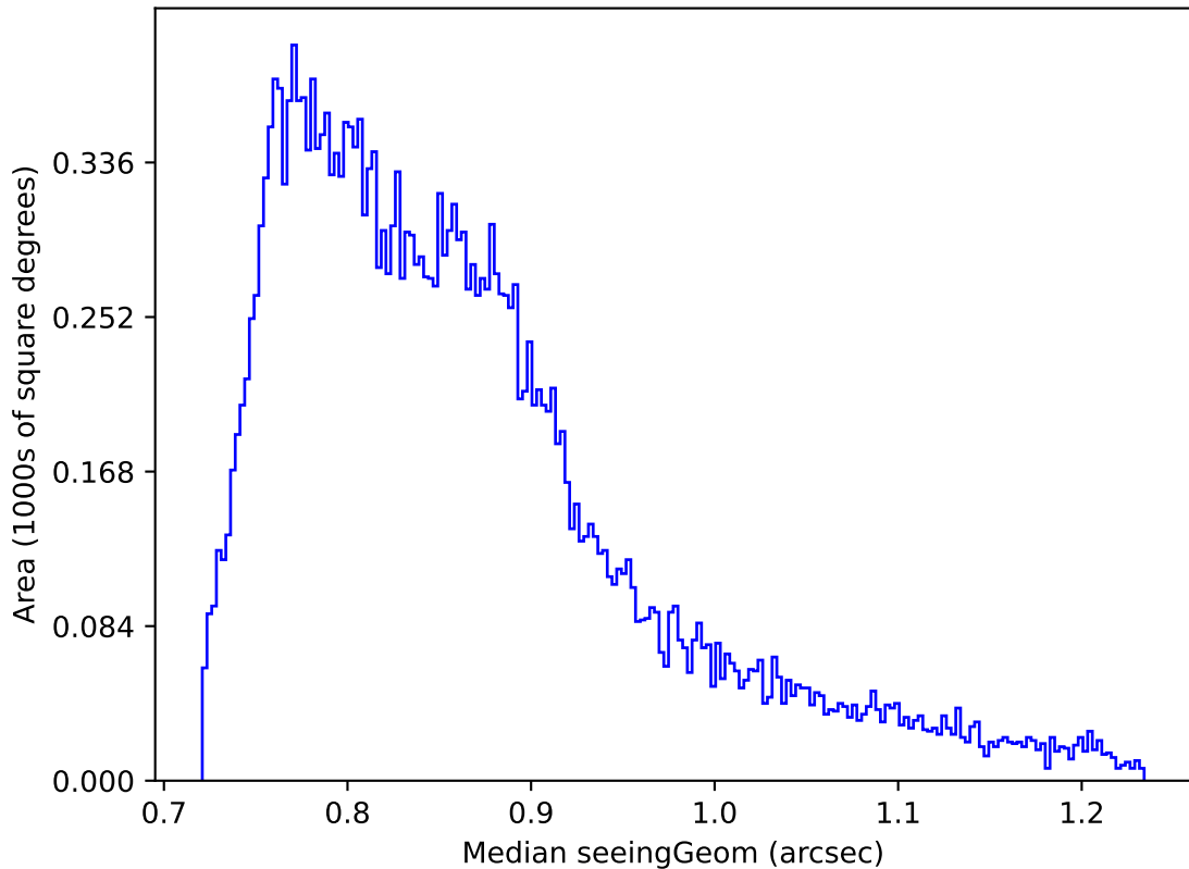
roll_pause_mjdp0_v3.4_10yrs Yr 1 all bands: Median seeingGeom
