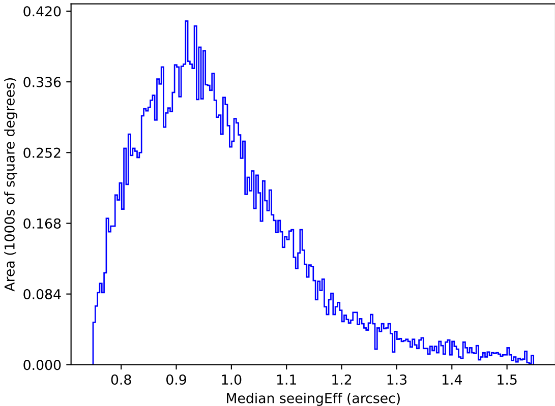
roll_pause_mjdp0_v3.4_10yrs Yr 1 z band: Median seeingEff
