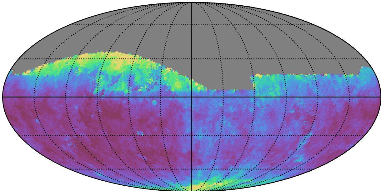
roll_pause_mjdp0_v3.4_10yrs Yr 1 all bands: Median seeingEff
