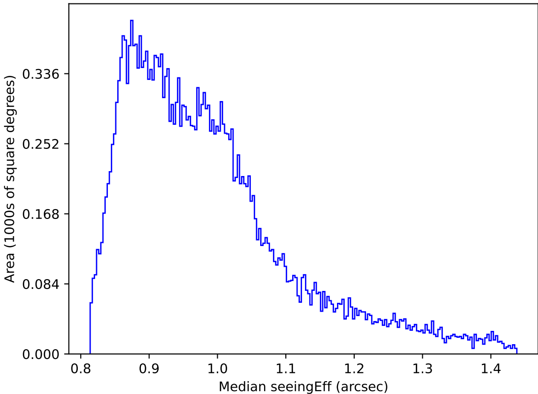
roll_pause_mjdp0_v3.4_10yrs Yr 1 all bands: Median seeingEff
