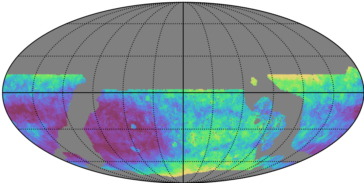
roll_pause_mjdp0_v3.4_10yrs WFD z band: Median seeingEff
