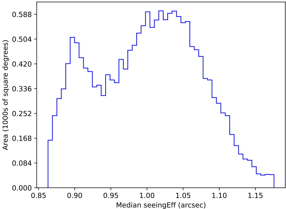
roll_pause_mjdp0_v3.4_10yrs WFD z band: Median seeingEff
