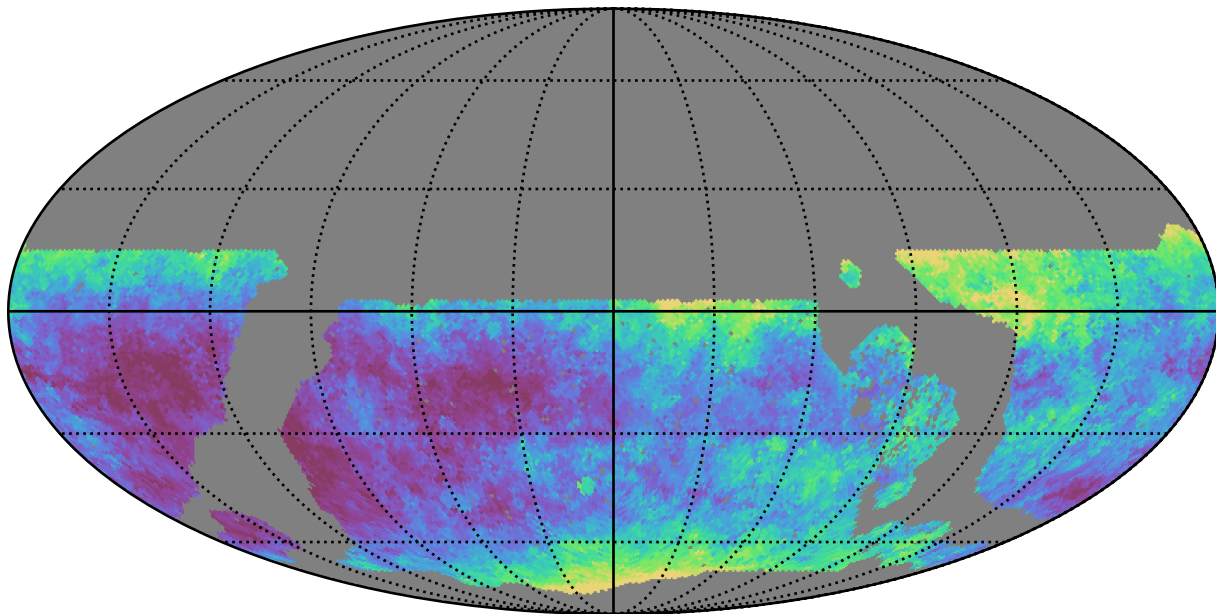
roll_pause_mjdp0_v3.4_10yrs WFD y band: Median seeingEff
