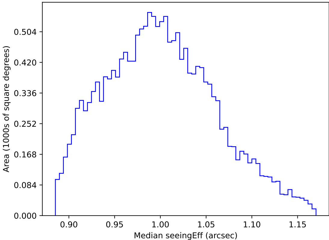
roll_pause_mjdp0_v3.4_10yrs WFD y band: Median seeingEff
