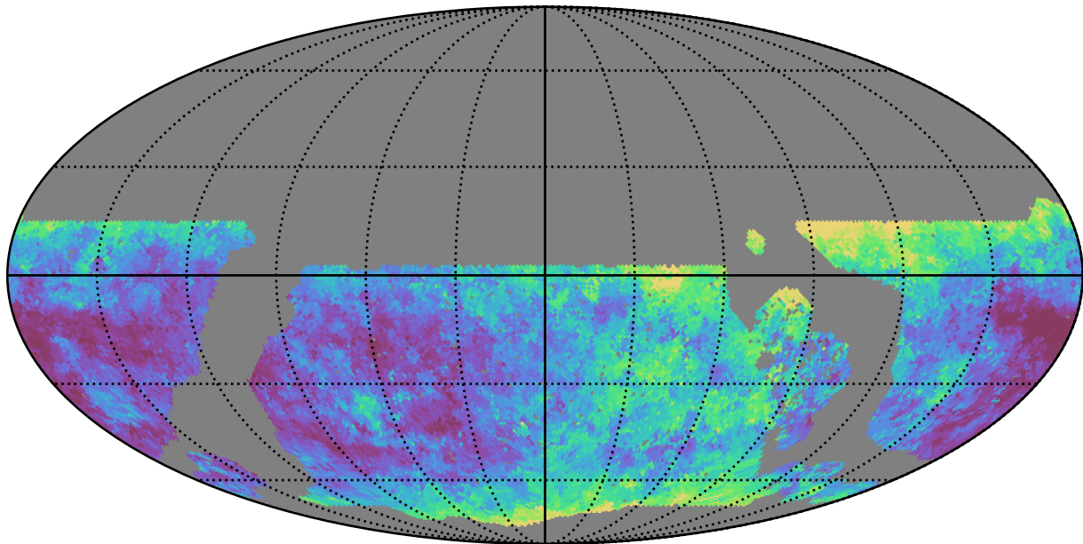
roll_pause_mjdp0_v3.4_10yrs WFD u band: Median seeingEff
