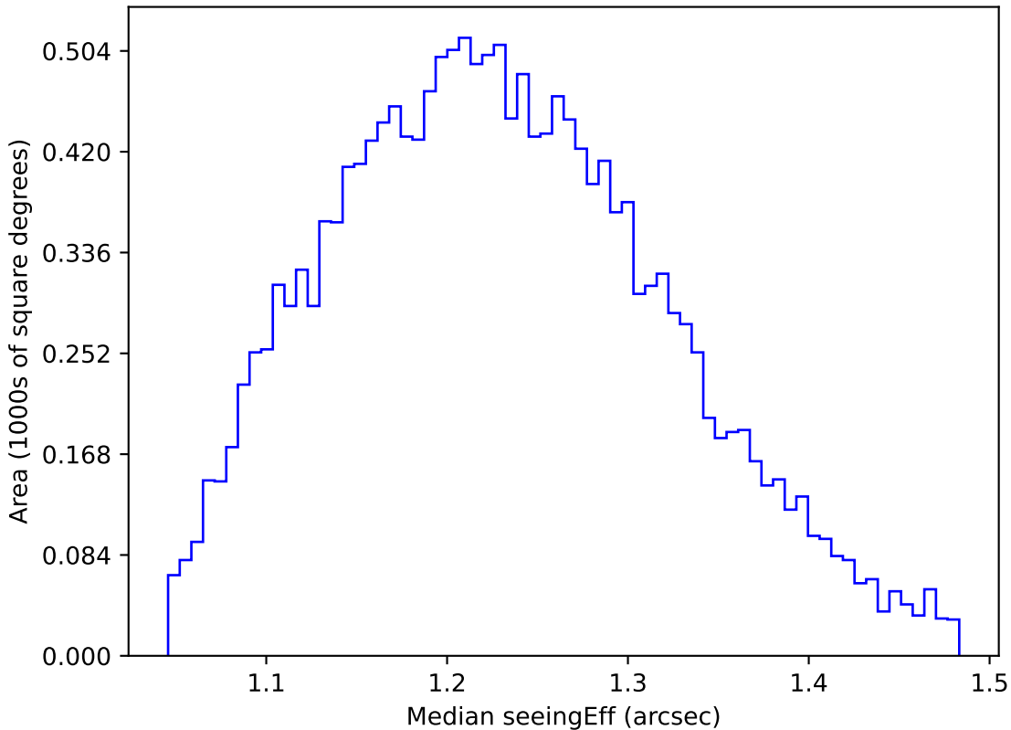
roll_pause_mjdp0_v3.4_10yrs WFD u band: Median seeingEff
