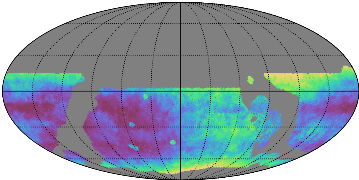
roll_pause_mjdp0_v3.4_10yrs WFD r band: Median seeingEff
