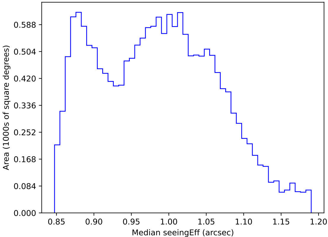
roll_pause_mjdp0_v3.4_10yrs WFD i band: Median seeingEff
