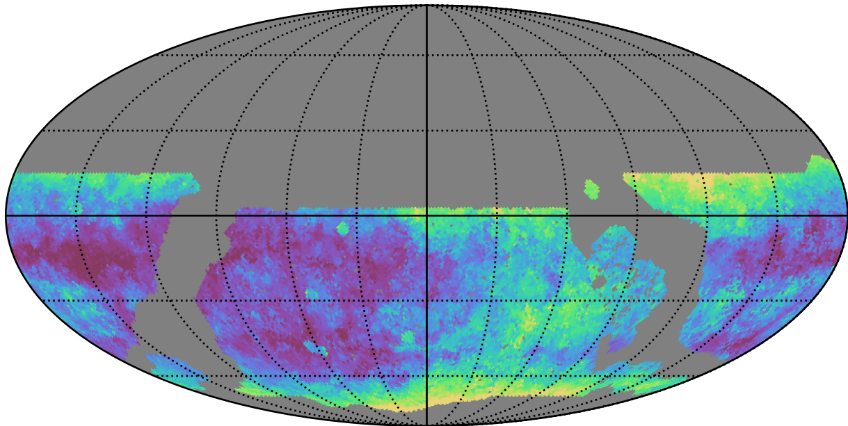
roll_pause_mjdp0_v3.4_10yrs WFD g band: Median seeingEff
