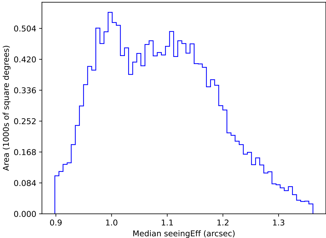
roll_pause_mjdp0_v3.4_10yrs WFD g band: Median seeingEff
