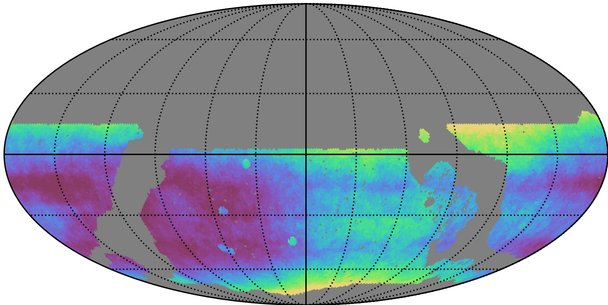
roll_pause_mjdp0_v3.4_10yrs WFD all bands: Median seeingEff
