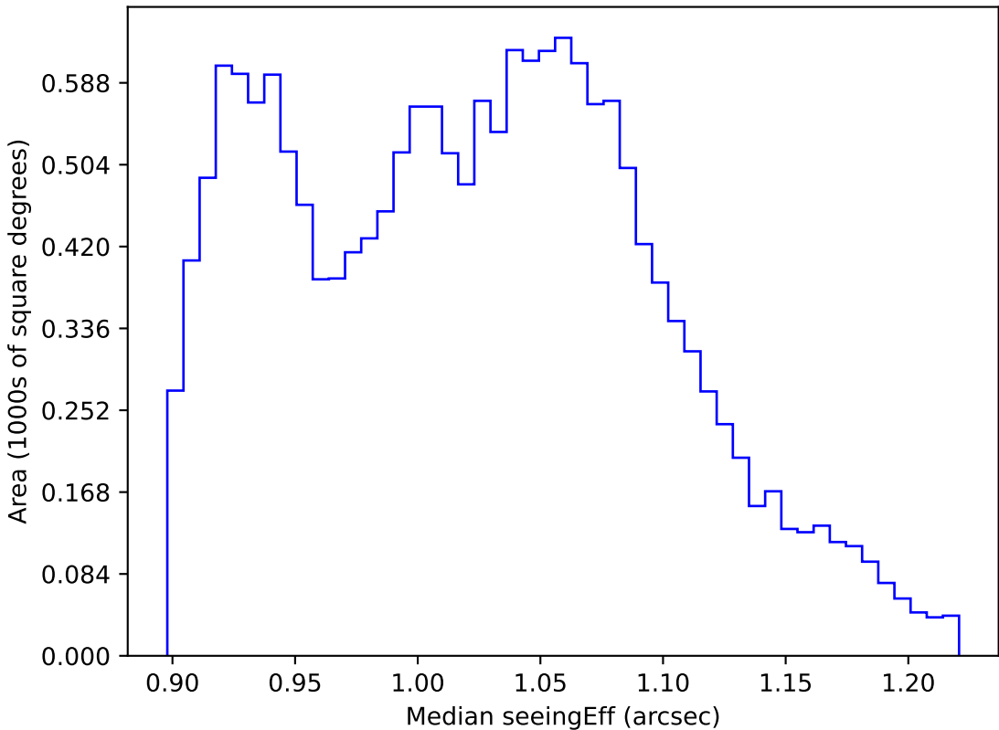
roll_pause_mjdp0_v3.4_10yrs WFD all bands: Median seeingEff
