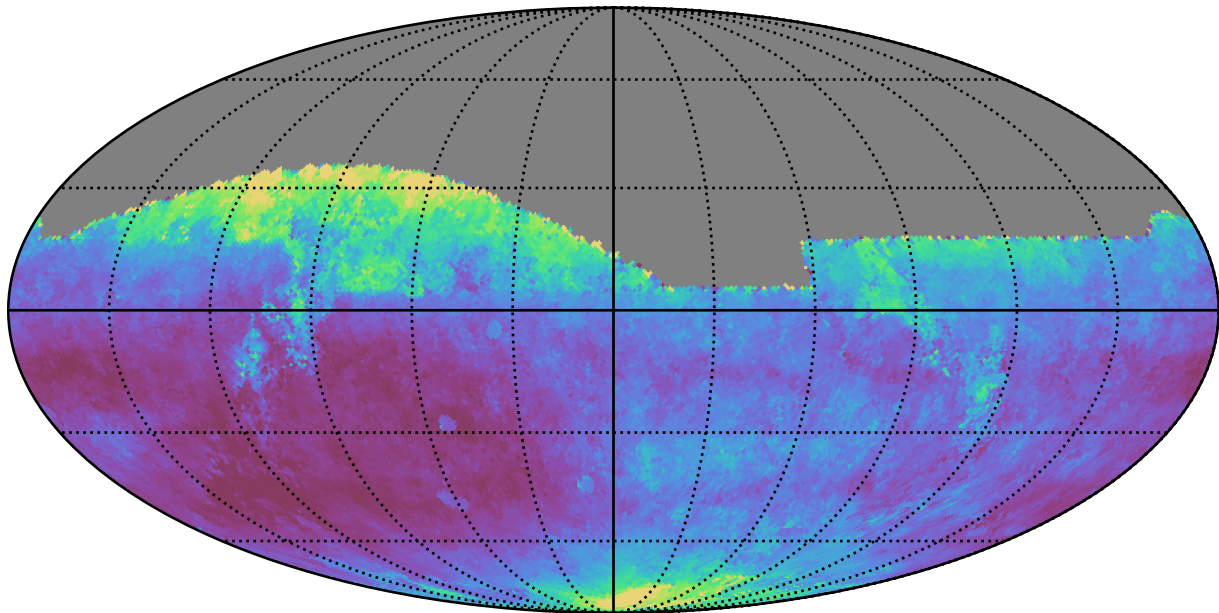
roll_pause_mjdp0_v3.4_10yrs All sky z band: Median seeingEff
