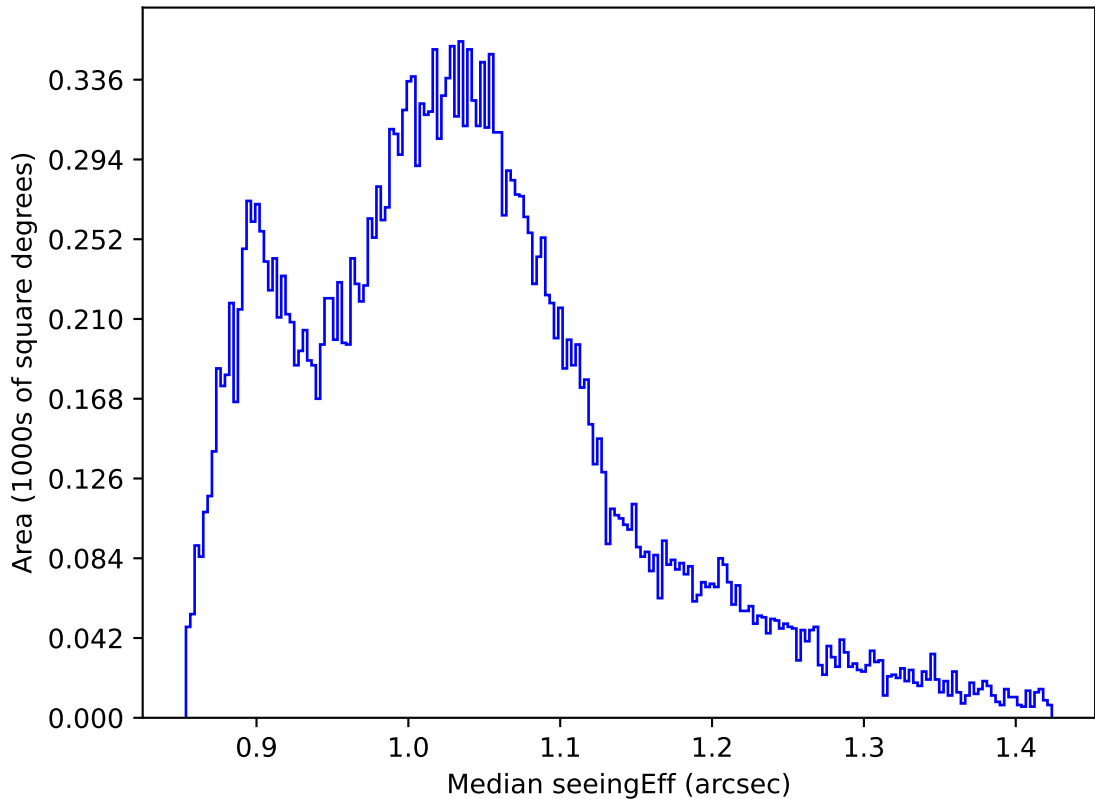
roll_pause_mjdp0_v3.4_10yrs All sky z band: Median seeingEff
