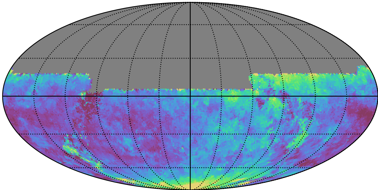
roll_pause_mjdp0_v3.4_10yrs All sky u band: Median seeingEff
