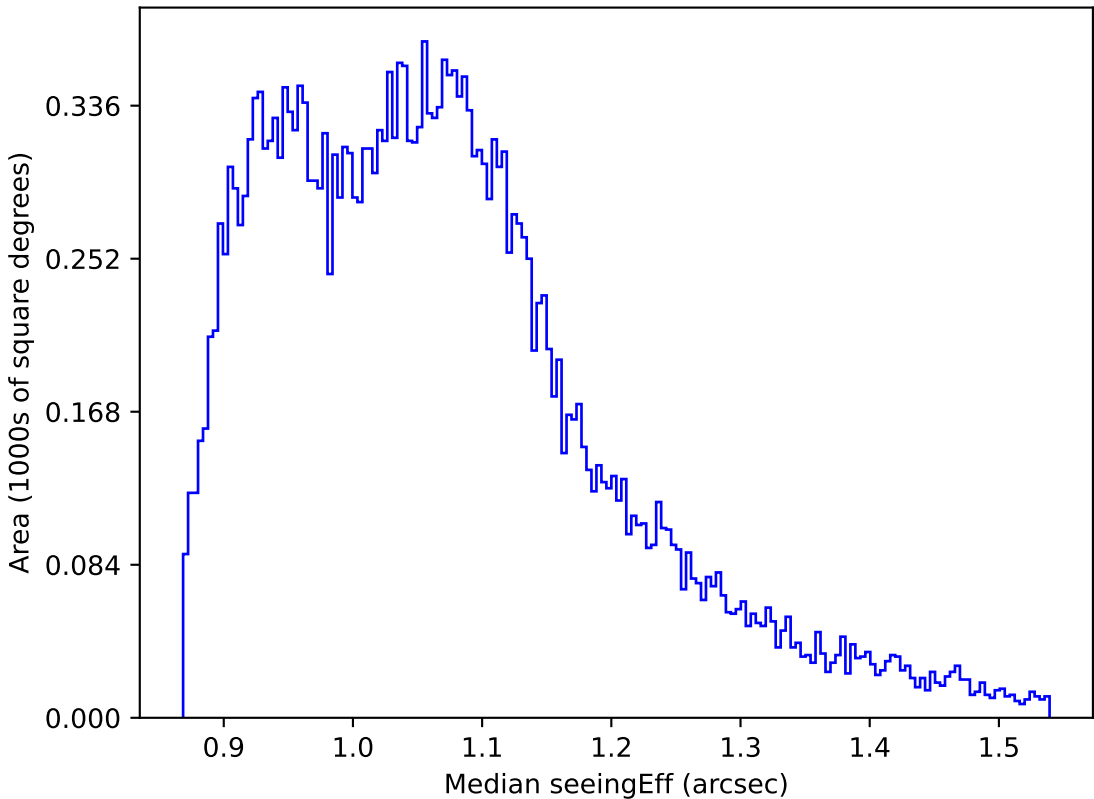
roll_pause_mjdp0_v3.4_10yrs All sky r band: Median seeingEff
