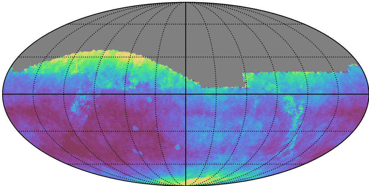
roll_pause_mjdp0_v3.4_10yrs All sky i band: Median seeingEff
