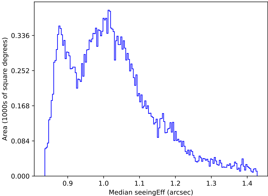
roll_pause_mjdp0_v3.4_10yrs All sky i band: Median seeingEff
