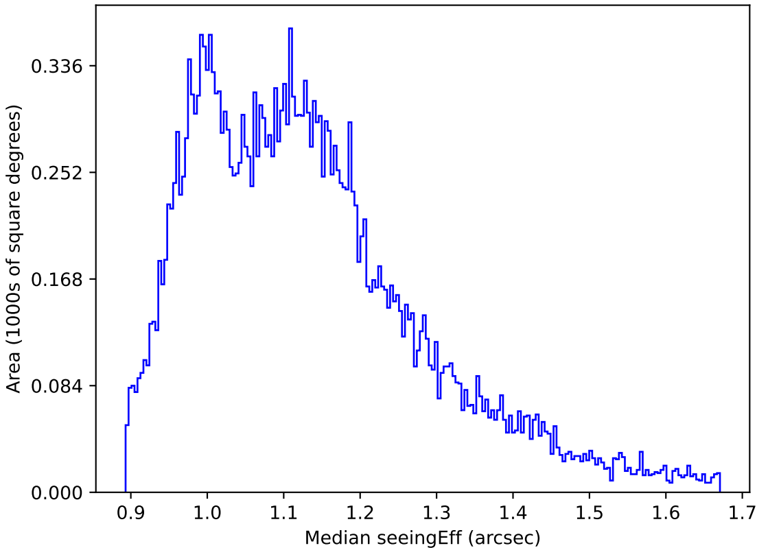
roll_pause_mjdp0_v3.4_10yrs All sky g band: Median seeingEff
