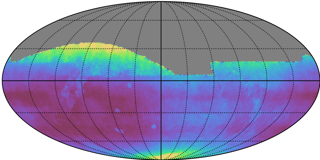
roll_pause_mjdp0_v3.4_10yrs All sky all bands: Median seeingEff
