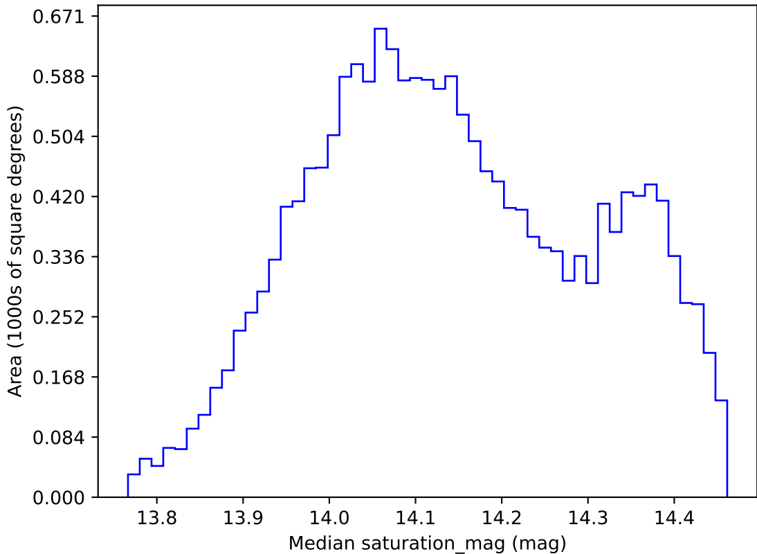
roll_pause_mjdp0_v3.4_10yrs WFD z band: Median saturation_mag
