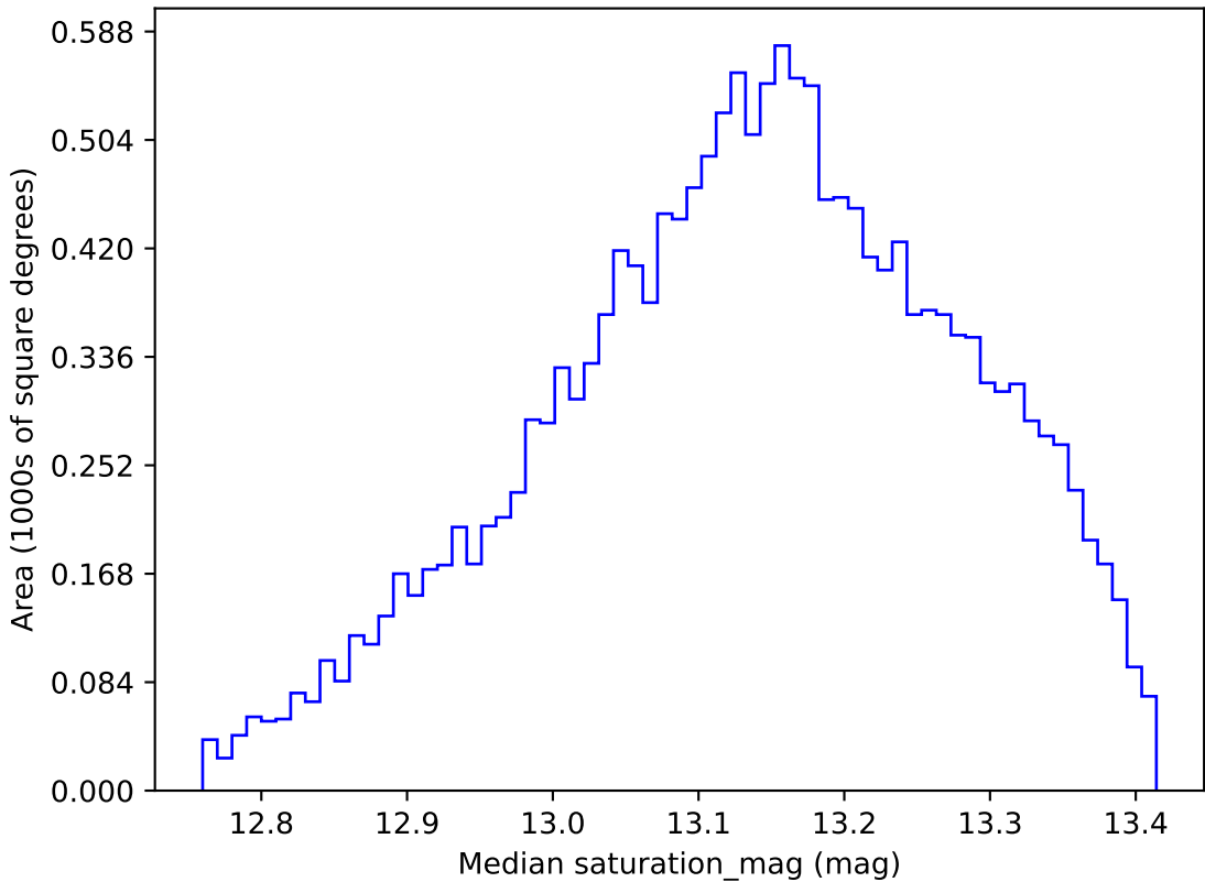
roll_pause_mjdp0_v3.4_10yrs WFD y band: Median saturation_mag
