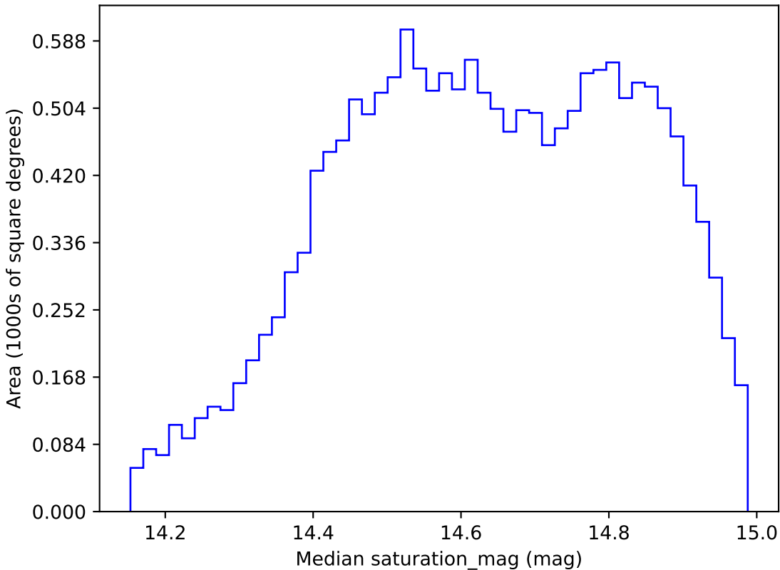
roll_pause_mjdp0_v3.4_10yrs WFD r band: Median saturation_mag
