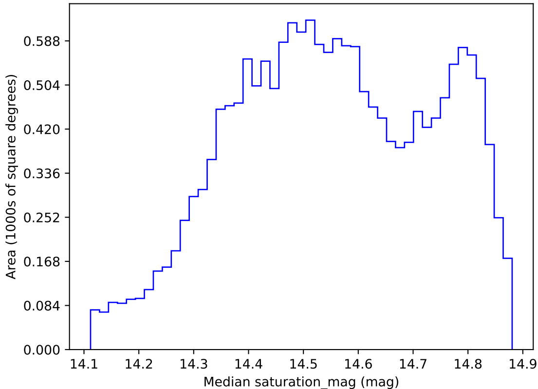
roll_pause_mjdp0_v3.4_10yrs WFD i band: Median saturation_mag
