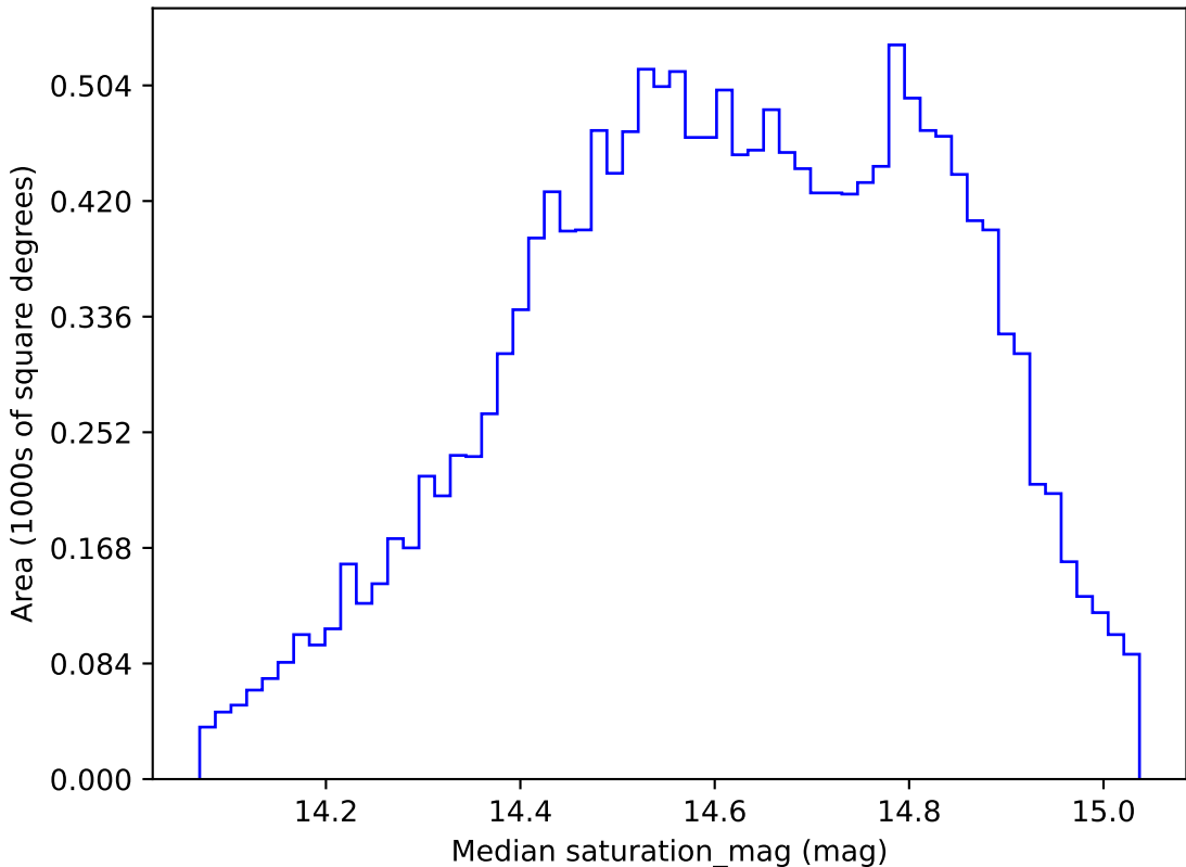
roll_pause_mjdp0_v3.4_10yrs WFD g band: Median saturation_mag
