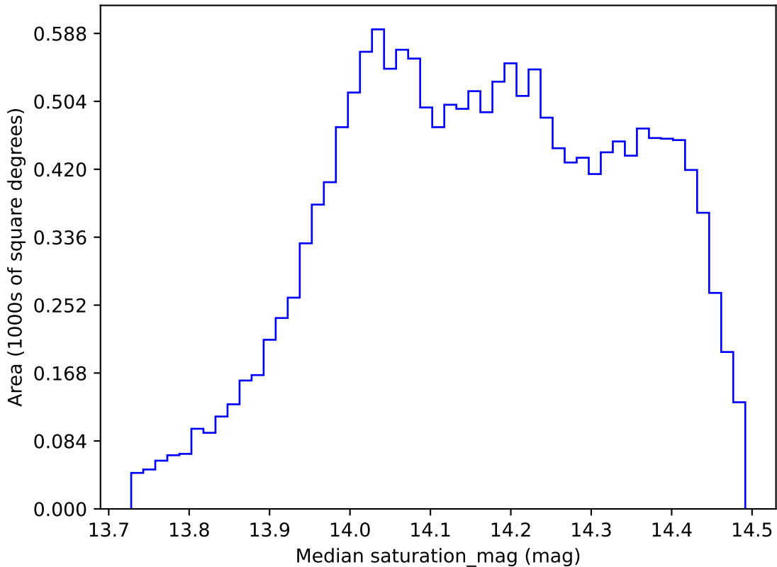
roll_pause_mjdp0_v3.4_10yrs WFD all bands: Median saturation_mag
