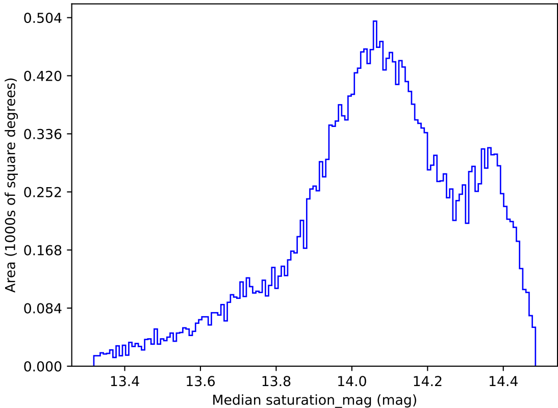
roll_pause_mjdp0_v3.4_10yrs All sky z band: Median saturation_mag
