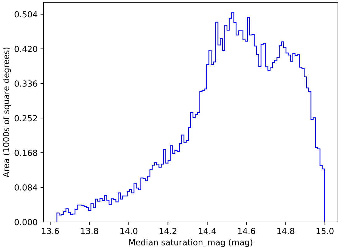
roll_pause_mjdp0_v3.4_10yrs All sky r band: Median saturation_mag
