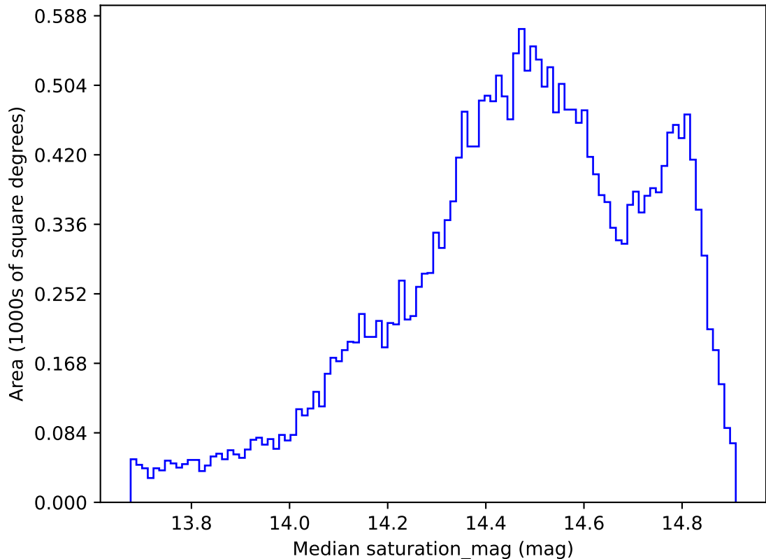
roll_pause_mjdp0_v3.4_10yrs All sky i band: Median saturation_mag
