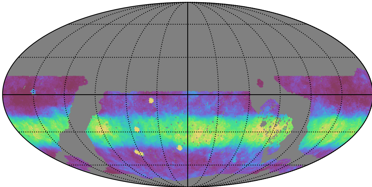
roll_pause_mjdp0_v3.4_10yrs WFD z band: Median normairmass
