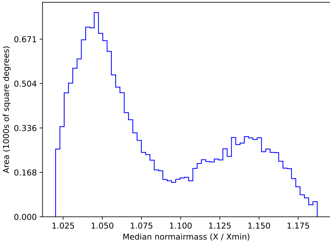
roll_pause_mjdp0_v3.4_10yrs WFD z band: Median normairmass
