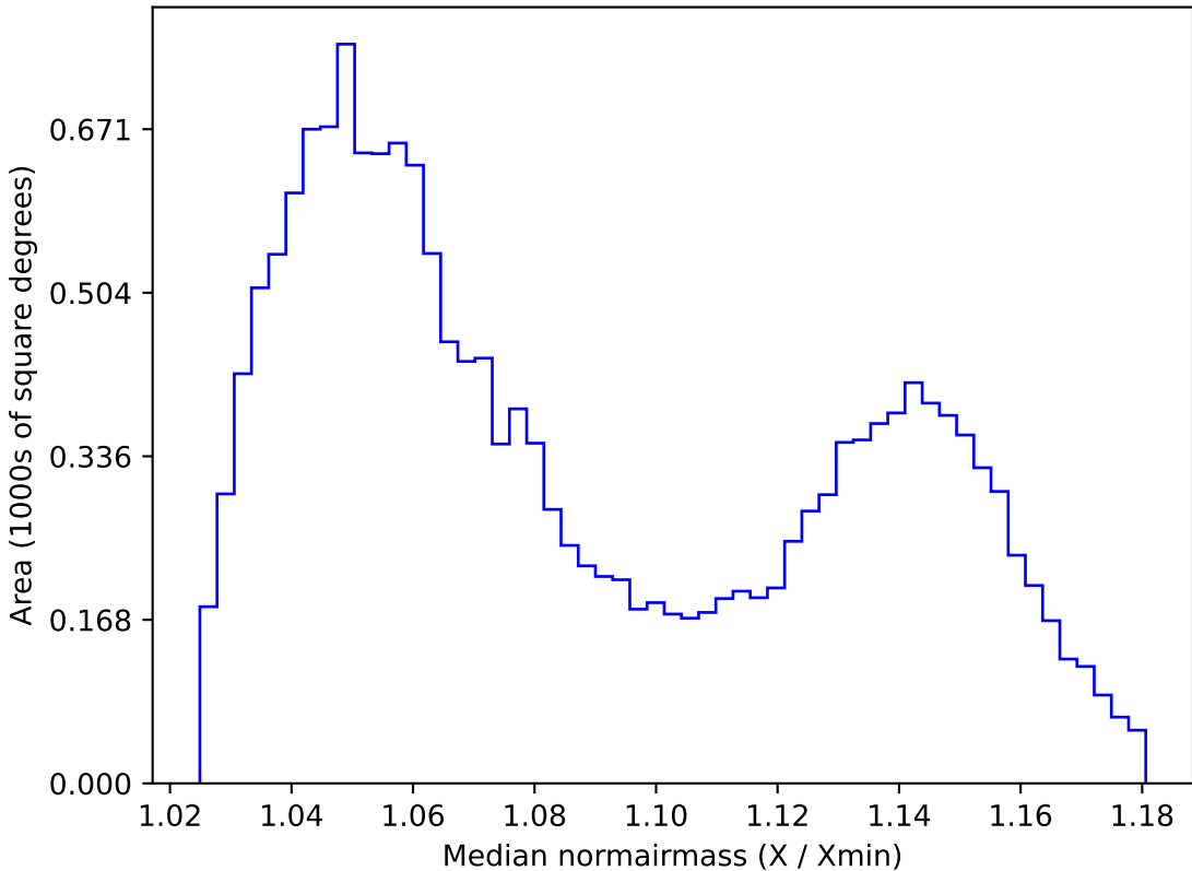
roll_pause_mjdp0_v3.4_10yrs WFD y band: Median normairmass
