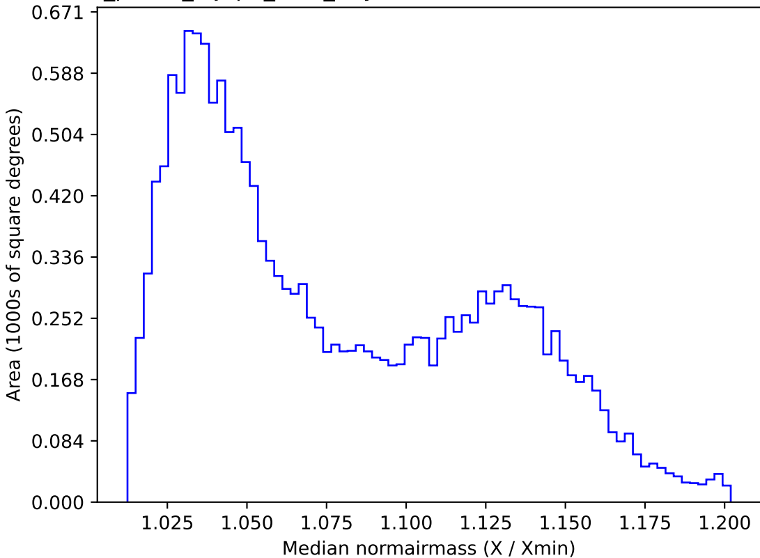
roll_pause_mjdp0_v3.4_10yrs WFD u band: Median normairmass
