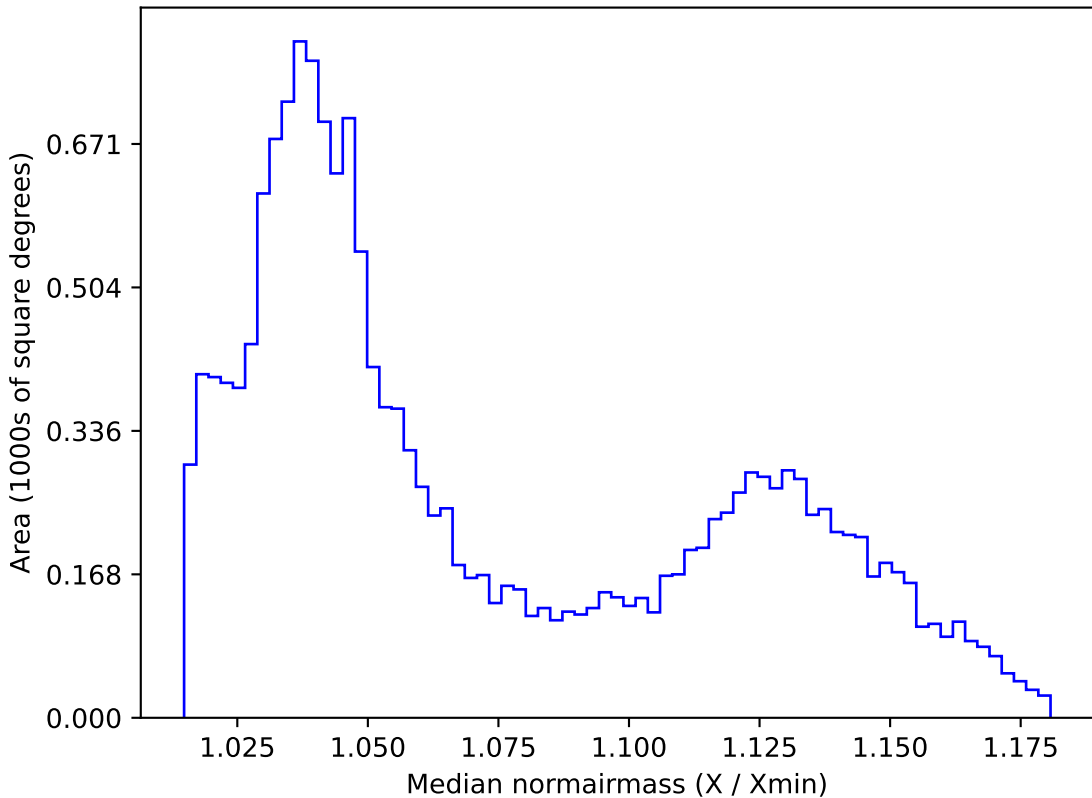
roll_pause_mjdp0_v3.4_10yrs WFD r band: Median normairmass
