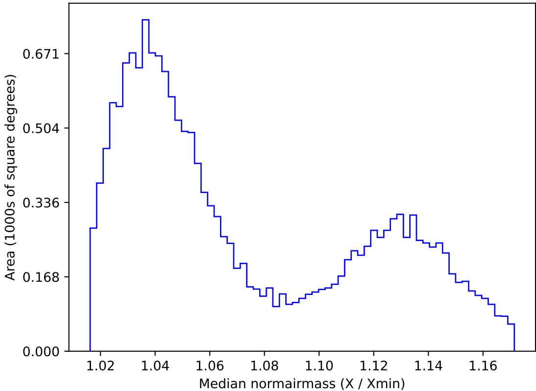
roll_pause_mjdp0_v3.4_10yrs WFD i band: Median normairmass
