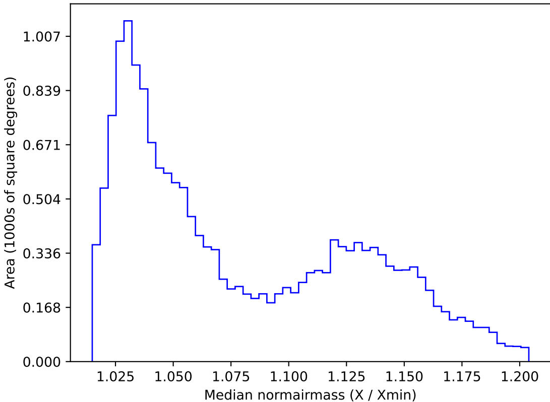
roll_pause_mjdp0_v3.4_10yrs WFD g band: Median normairmass
