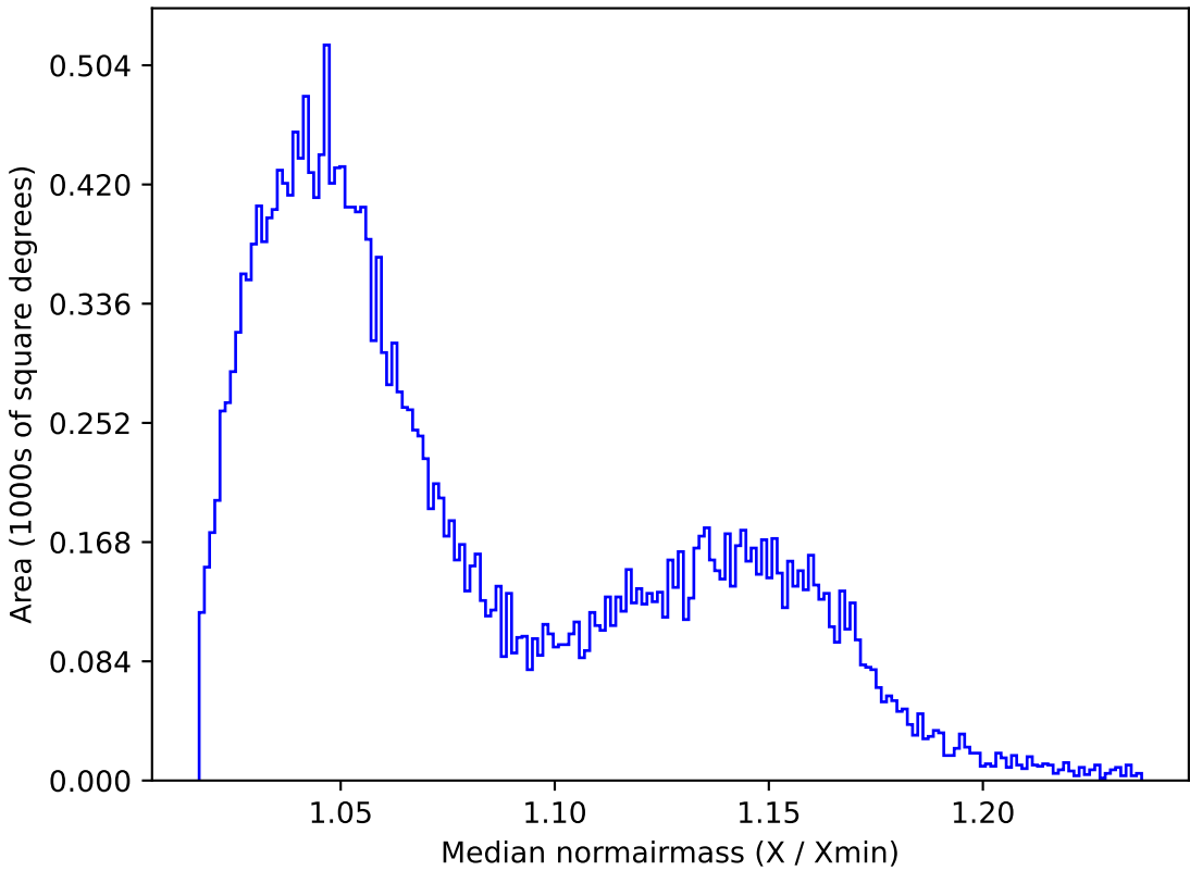
roll_pause_mjdp0_v3.4_10yrs All sky z band: Median normairmass
