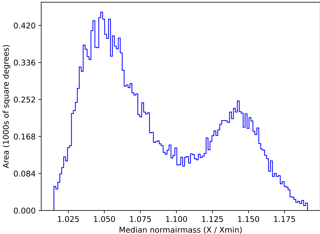
roll_pause_mjdp0_v3.4_10yrs All sky y band: Median normairmass
