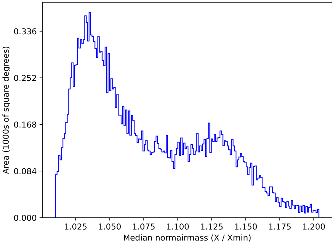
roll_pause_mjdp0_v3.4_10yrs All sky u band: Median normairmass
