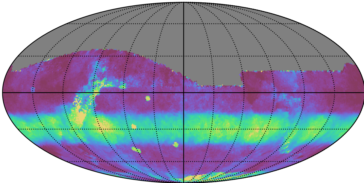
roll_pause_mjdp0_v3.4_10yrs All sky r band: Median normairmass
